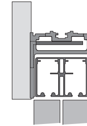
Binario a parete / Wall rail
