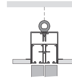
Binario a soffitto in cartongesso / Ceiling rail in plasterboard
