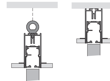
Binario a soffitto in cartongesso / Ceiling rail in plasterboard
