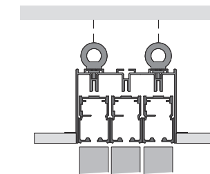
Binario a soffitto in cartongesso / Ceiling rail in plasterboard
