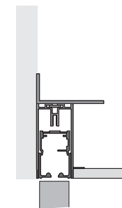
Binario a parete cartongesso / Wall rail in plasterboard
