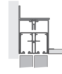
Binario a parete cartongesso / Wall rail in plasterboard
