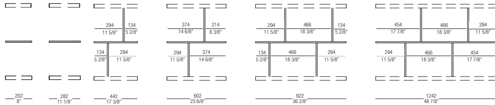
Raster
