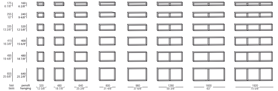
Contenitori base e standard - P 384 - 490 / Contenitori pensili P 384 Base containers e standard - D 15 1/8"-19 2/8" / Hanging containers D 15 1/8"
