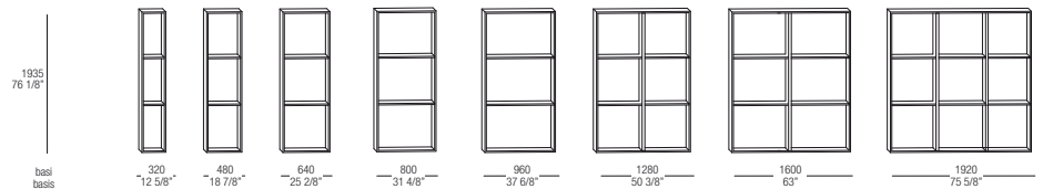
Contenitori base e standard - P 384 - 490 / Contenitori pensili P 384 Base containers e standard - D 15 1/8"-19 2/8" / Hanging containers D 15 1/8"
