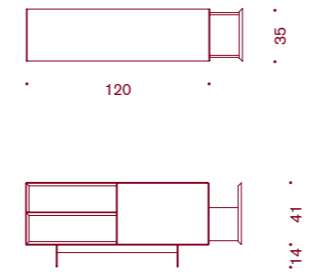
LIBRERIA H 65 E H 75 BOOKCASE H 65 AND H 75
