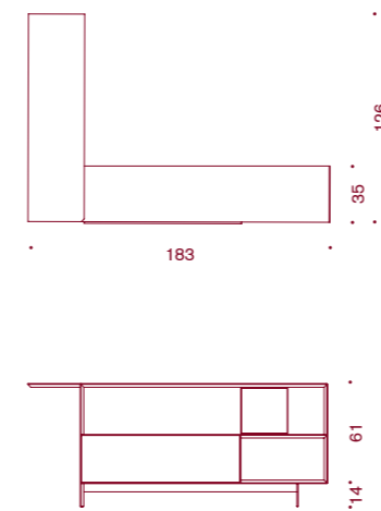
LIBRERIA CON WORK TOP H 75 BOOKCASE WITH DESK H 75
